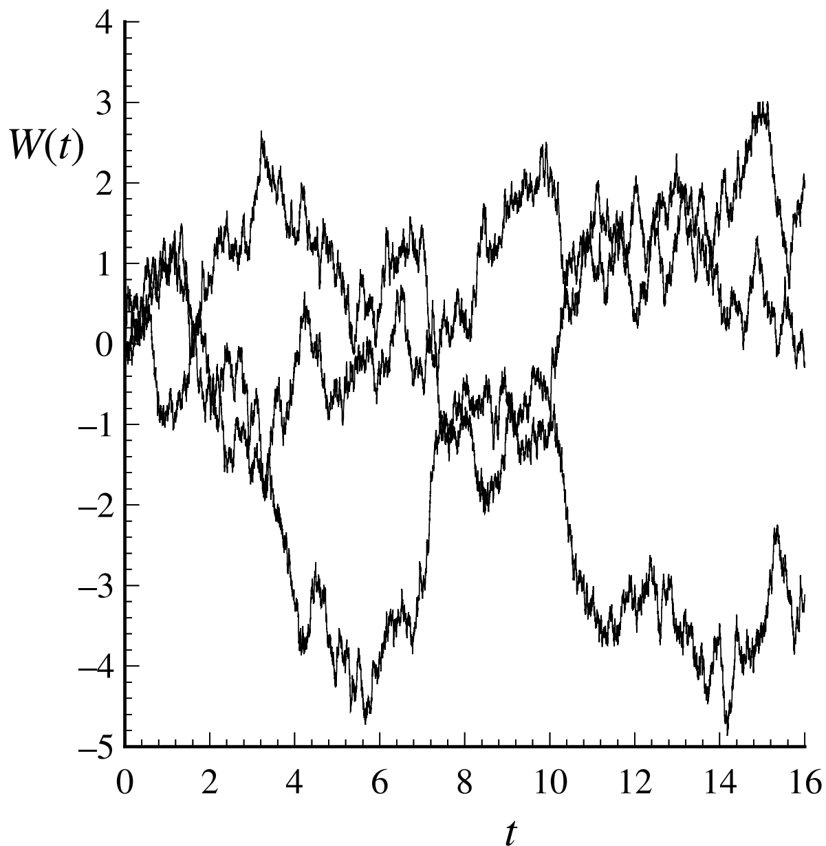
Figure J.1: Three sample paths of the Wiener process.
